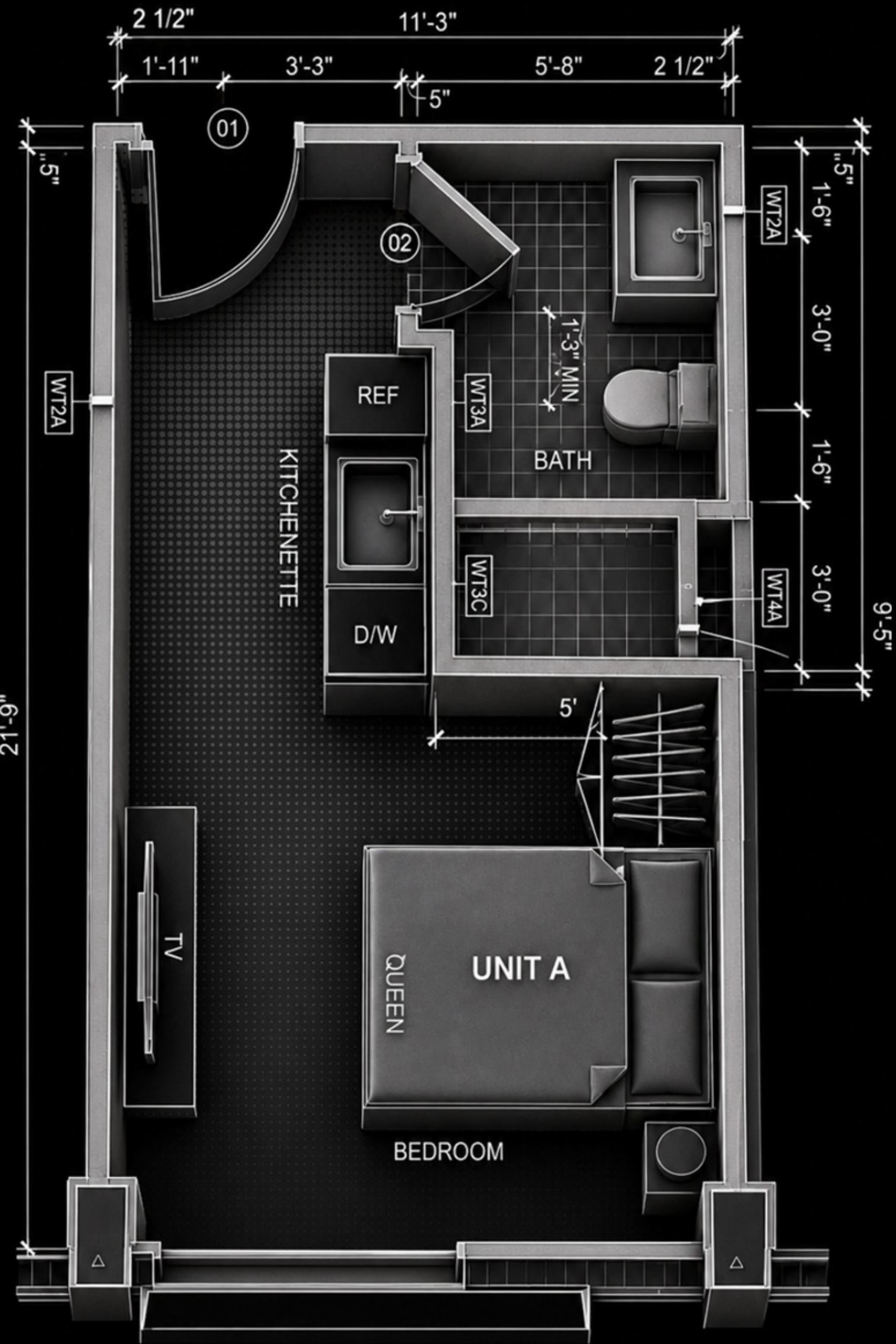
1 A-200 UNIT A_ENLARGED PLAN SCALE: 1/4" = 1'-0"
